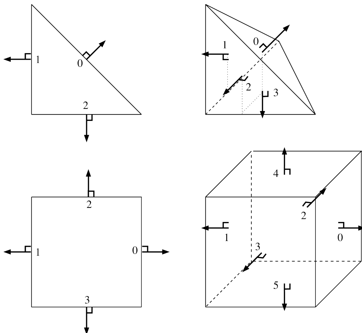
Fig. 7: Example of RT0 elements in dimension two and three. The RT k element on a simplex of dimension P and degree K has \frac{(K + P - 1)!}{K!(P - 1)!} normal component degrees of freedom on each face and \frac{K(K + P - 1)!}{K!(P - 1)!} internal Lagrange degrees of freedom. For the quadrilateral, only the lowest degree element is implemented yet.
