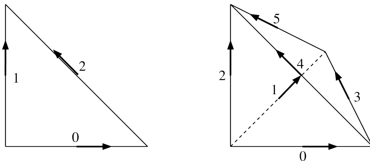
Fig. 8: Nedelec edge elements in dimension two and three. (P(P+1)/2 dof, H(\text{rot}))
